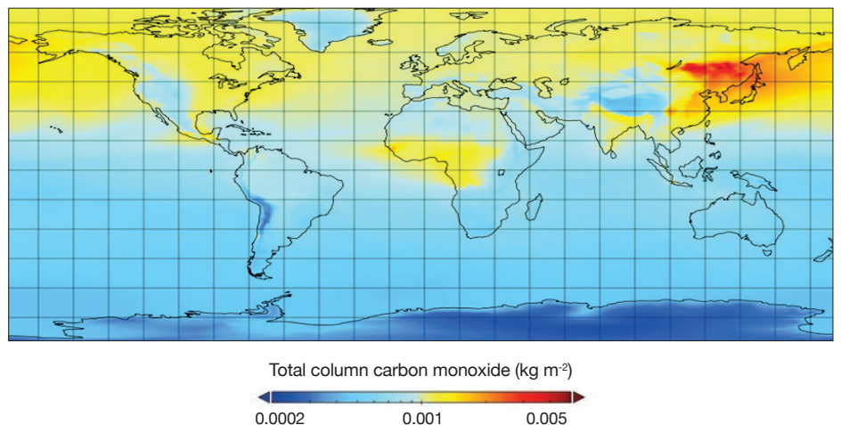
CAMS global reanalysis for carbon monoxide averaged over May 2003.
