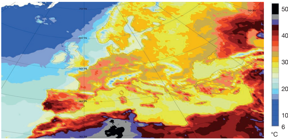
Maximum temperature in Europe, ECMWF analysis between 29 July & 6 August 2018
