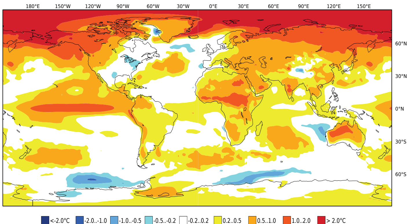
Example of a C3S multi-system seasonal forecast for mean 2m temperature anomaly
